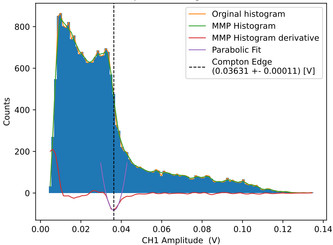
CH1 Amplitude histogram for 43.5V
