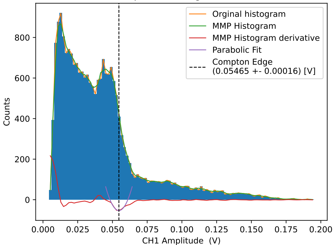
CH1 Amplitude histogram for 45.0V
