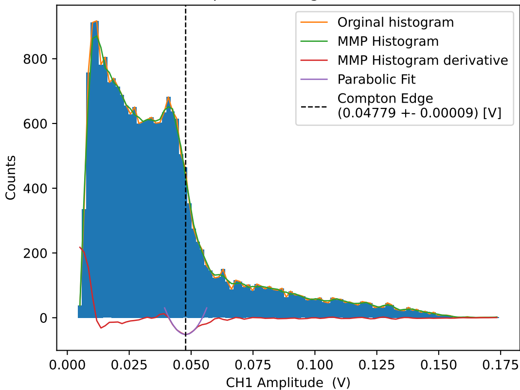
CH1 Amplitude histogram for 44.5V
