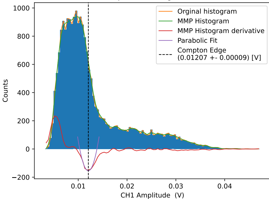
CH1 Amplitude histogram for 41V
